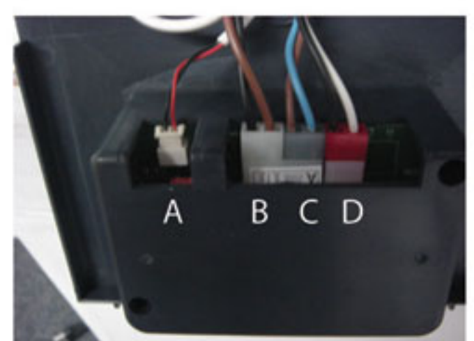
Insert 4 pin connectors into new Digital Controller. Color Sequence: Left to Right Small White Pin : A Md. White Pin: B Md. Blue Pin: C Md. Red Pin: D
